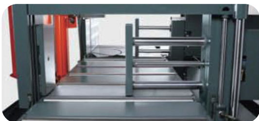
Full stroke hydraulic vises & servo motor driven shuttle bed
